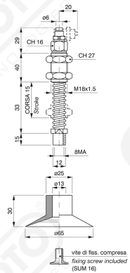
Art. PS 65/1 C. 15 x art. VSP 65/1
