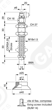
Art. PS 40/1 C. 25 x art. VSP 40/1
